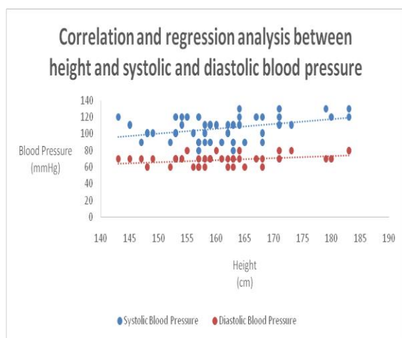
Figure 1: Correlation and regression analysis between height and systolic and diastolic blood pressure
